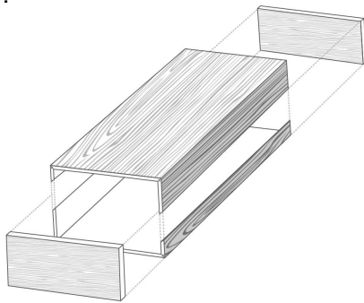
Mitred L-shape double sided
