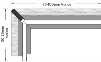
Flush mitre with metal trim
