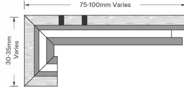
Overhung return mitre with metal tactile indicator
